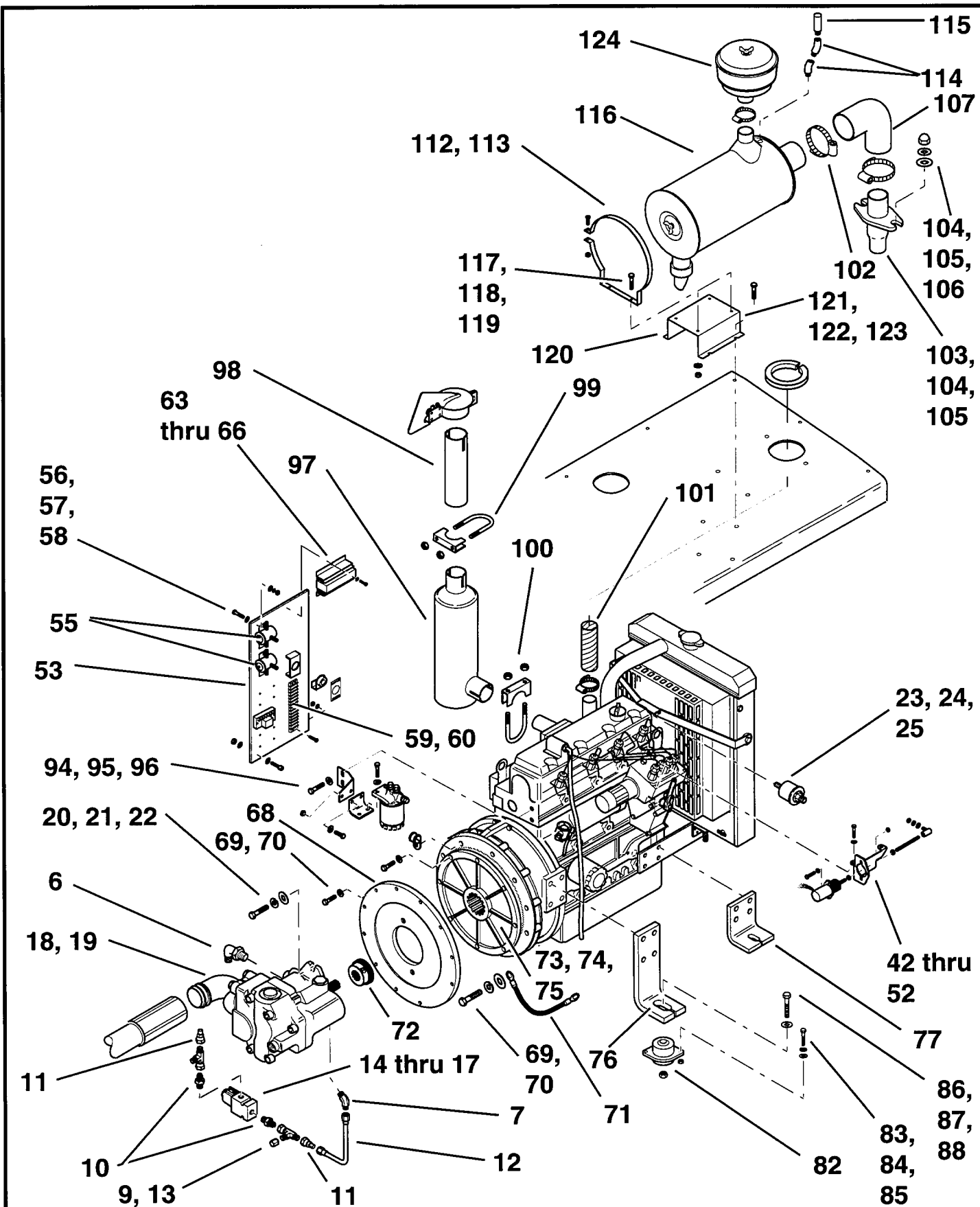
TITLE ENGINE ASSEMBLY, DETROIT DIESEL/ PERKINS 104.22 (PLATE 1 OF 5)
